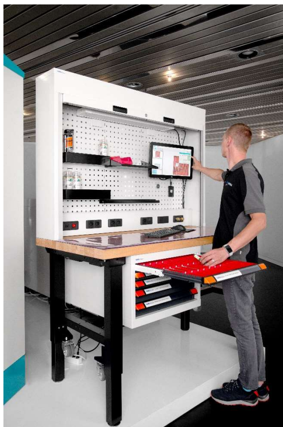
Quattro workstation with SmartBox
